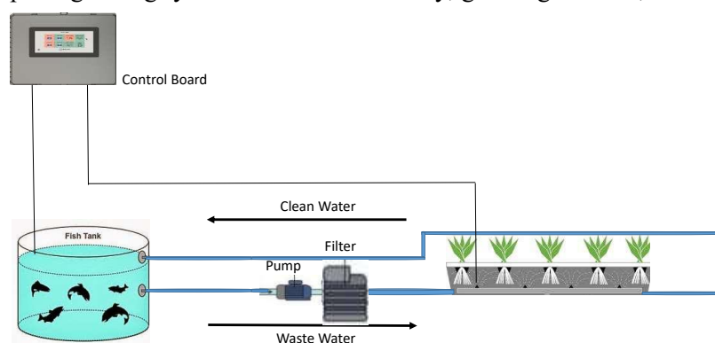
Figure. Representation of a coupled aquaponics system
