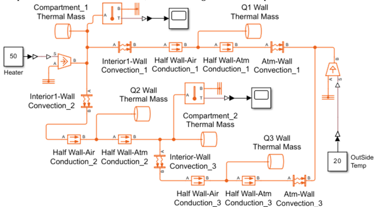
Figure 1. Simscape model of the two-room example with one heater
